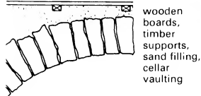
wooden boarded floor above cellar vaulting
